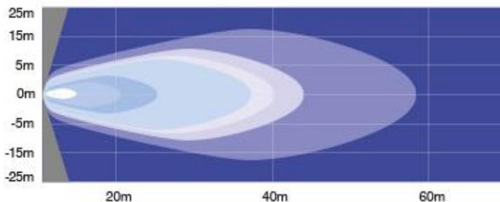
MLB-12-60: 60° Extra Wide Beam Pattern
