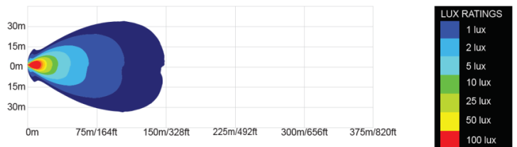
MLPR-84-40 – Flood Beam Pattern
