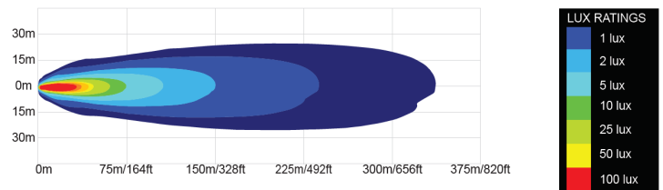
MLPR-84-10 – Spot Beam Pattern
