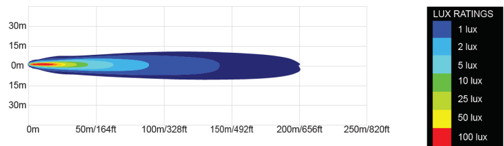
MLPR-35-10 – Spot Beam Pattern
