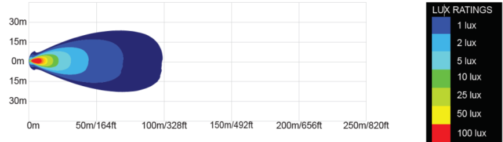
MLPR-35-40 – Flood Beam Pattern
